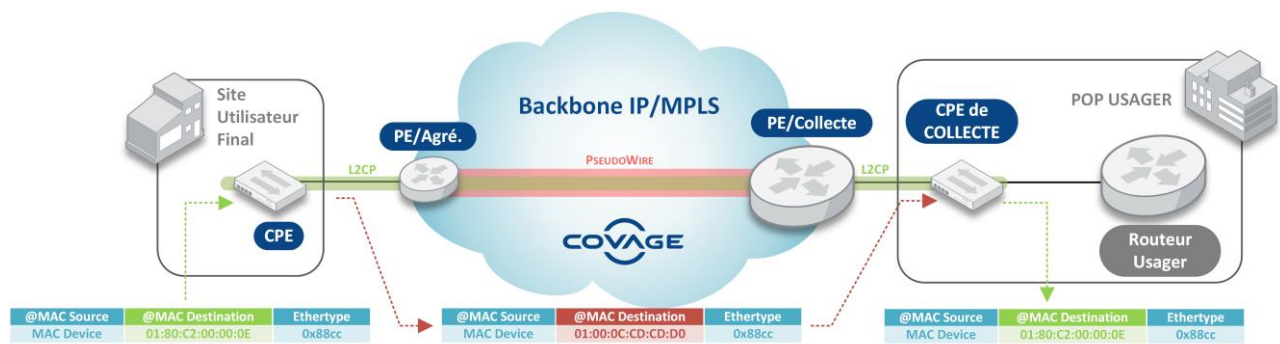
Figure 6 - Transparence Protocolaire : L2CP
